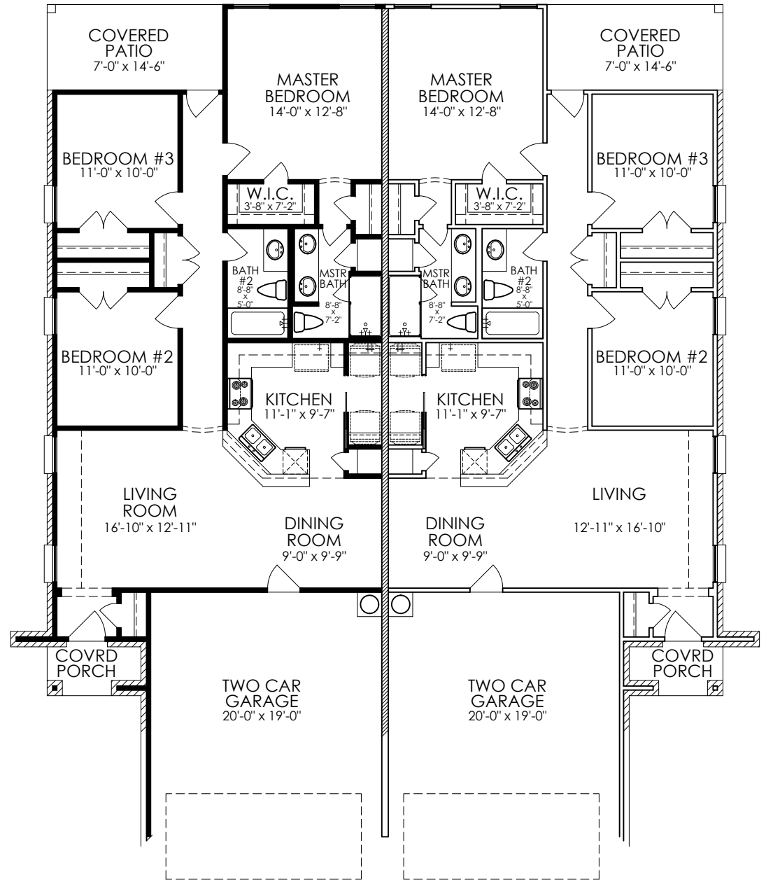
FLOOR PLAN
